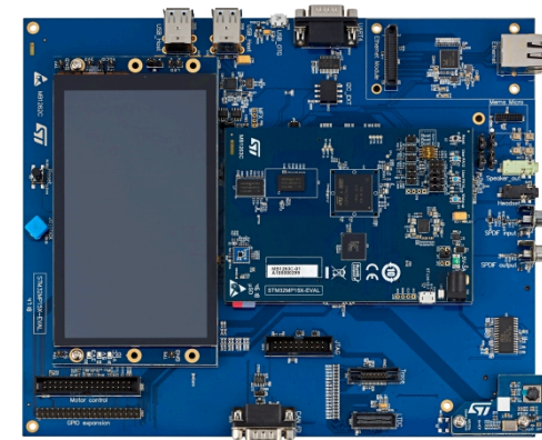
STM32MP157C-EV1 eval board
