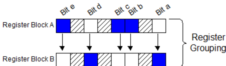
Fig. 4.5: Example Fixed Hardware Feature Register Grouping
