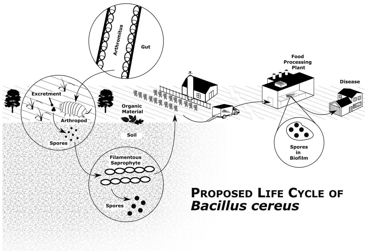
Figure 2. Proposed life cycle of Bacillus cereus . B. cereus spores germinate within an animal host and enter soil through droppings or carcasses or they germinate on contact with organic material. Saprophytic growth occurs in soil. Cells/spores contaminate plant material and food processing areas (where spores persist, especially in biofilms) then cause disease after human consumption. 25–27
