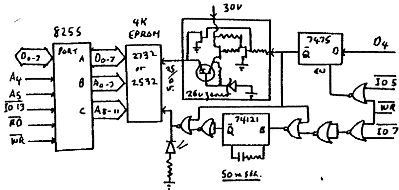
Fig 2 Eeprom programmer for the Ace.
