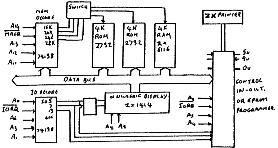
Fig 1 Ace Add-on for Eeprom expansion and instrument control.
