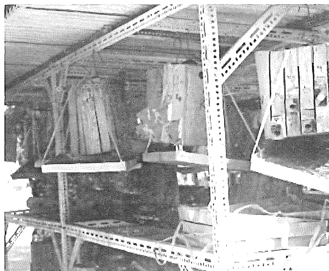
Nest hive boxes for Xylocopa , showing individual frames, tunnels made by bees (exposed for photograph) within a frame and placement of nest boxes in a bee shelter, suspended by wires
