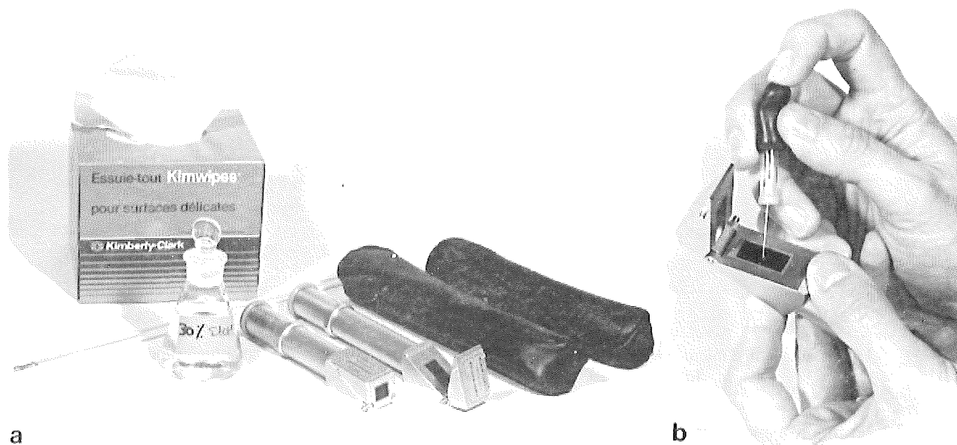
Fig. 13. a) instruments for determining nectar sugar concentration — refractometers and protective cases, thermometer, tissues and 30% alcohol for cleaning, b) method for applying nectar from microcapillary
