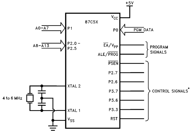
Figure 10. Programming the EPROM
