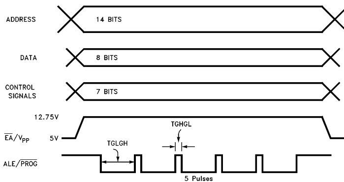
Figure 11. Programming Signal's Waveforms
