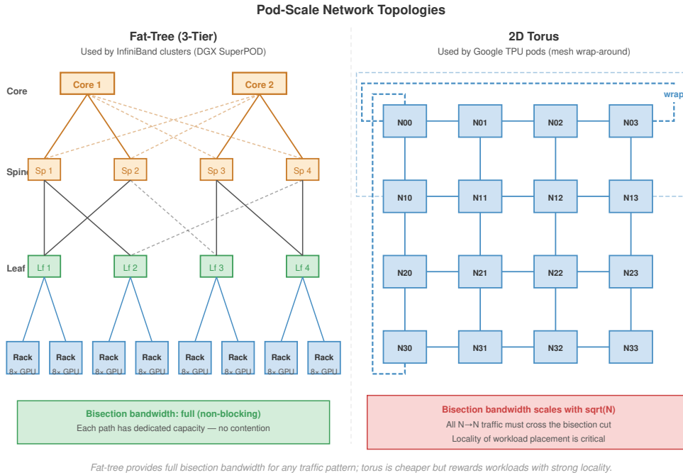
Figure 2.12: Pod-Scale Network Topologies: Two dominant pod topologies compared. (Left) Fat-Tree (3-Tier) with Leaf, Spine, and Core tiers: full bisection bandwidth, used by InfiniBand clusters such as DGX SuperPOD. (Right) 2D Torus with wrap-around links: bisection bandwidth scales as \mathcal{O}(\sqrt{N}) , cheaper at scale but rewards workloads with strong locality; used by Google TPU pods. The choice shapes which parallelism strategies run efficiently.
