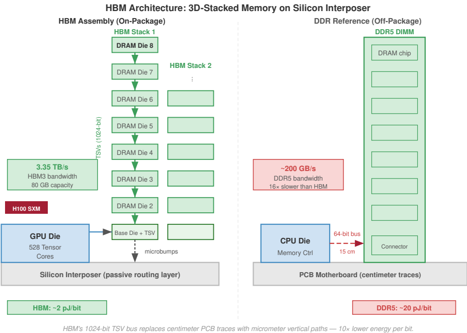
Figure 2.6: HBM 3D-Stacked Architecture: High Bandwidth Memory achieves its performance by vertically stacking DRAM dies and connecting them via Through-Silicon Vias (TSVs). The entire stack sits on a silicon interposer alongside the GPU die, enabling a 1024-bit-wide bus and reducing signal travel distance from centimeters to micrometers. This physical proximity is the key to breaking the memory wall.
