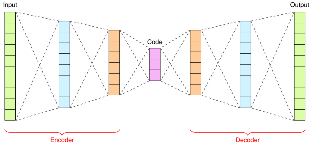
Figure 14.21: Autoencoder Architecture: Autoencoders learn compressed data representations by minimizing reconstruction error, enabling anomaly detection by identifying inputs with high reconstruction loss. During training on normal data, the network learns efficient encoding and decoding, making it sensitive to deviations indicative of potential poisoning attacks. Source: adapted from a Towards Data Science autoencoder tutorial.
