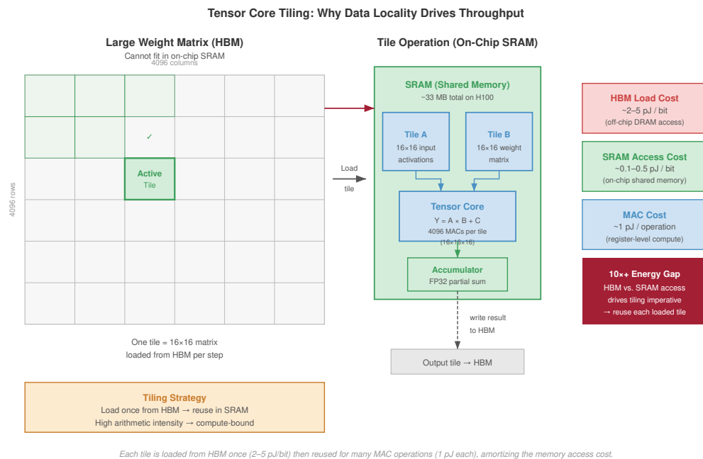
Figure 2.5: Tensor Core Tiling Strategy: To overcome the HBM bandwidth bottleneck, GPUs decompose large matrix operations into small tiles that fit within the Streaming Multiprocessor's (SM) fast SRAM. Data is loaded once into SRAM and reused across multiple Tensor Core operations, effectively multiplying the arithmetic value of every byte fetched from HBM.
