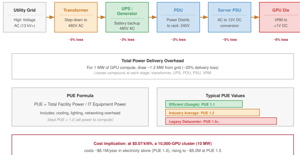
Figure 2.9: The Power Delivery Path: The journey of energy from the high-voltage grid to the low-voltage transistor involves multiple conversion stages, each with its own efficiency loss. The cumulative delivery loss, combined with overhead for cooling (measured by PUE), dictates how much power a facility must draw from the grid. The critical engineering challenge is the rack PDU to VRM transition, where 10–40 kW of power must be delivered within a single cabinet.
