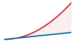
Huber loss caps the outlier influence that squared loss amplifies.
