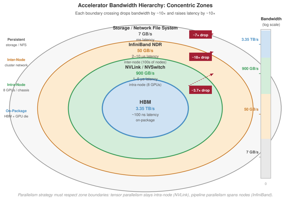
Figure 2.11: The Infrastructure Bandwidth Hierarchy: Concentric zones visualize the bandwidth tiers an ML workload crosses. HBM (3.35 TB/s) sits at the innermost zone; each outward boundary crossing drops bandwidth \sim 10\times and raises latency \sim 10\times : NVLink/NVSwitch (900 GB/s), InfiniBand NDR (50 GB/s), and Storage/Network File System (7 GB/s) at the outermost zone. Exploiting this hierarchy through tiered algorithms is the primary task of distributed systems engineering.
