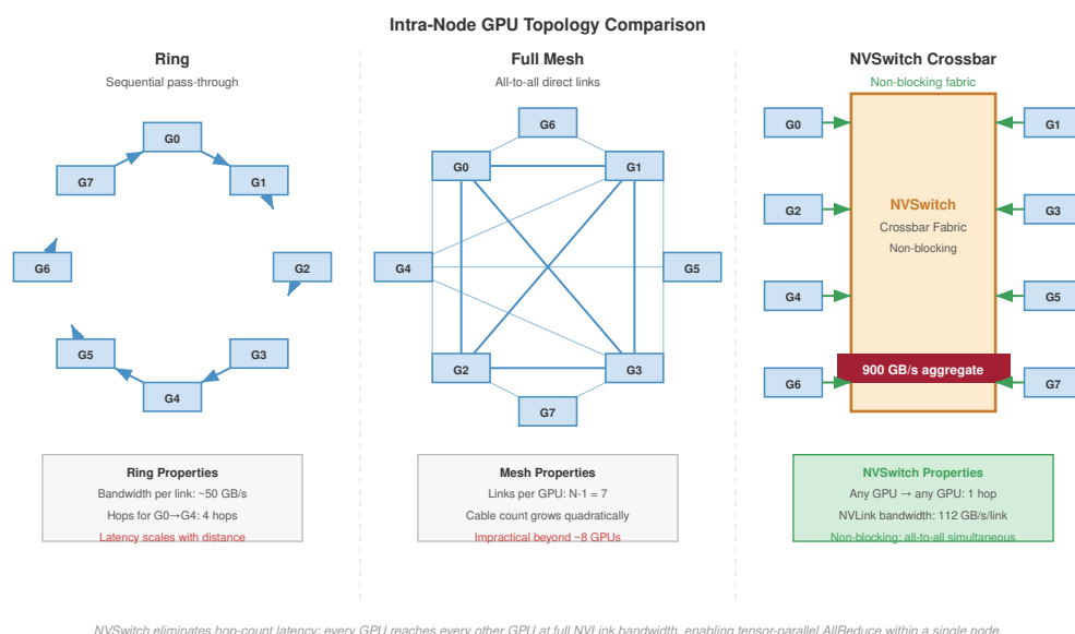
Figure 2.10: Intra-Node GPU Topology Comparison: Three approaches to wiring GPUs inside a node. (Left) Ring: sequential pass-through, ~50 GB/s per link, latency scales with distance. (Center) Full Mesh: all-to-all direct links, N - 1 links per GPU, impractical beyond ~8 GPUs. (Right) NVSwitch Crossbar: non-blocking fabric with 112 GB/s per NVLink and 900 GB/s aggregate, any-GPU-to-any-GPU in one hop, enabling tensor-parallel AllReduce within a node.
