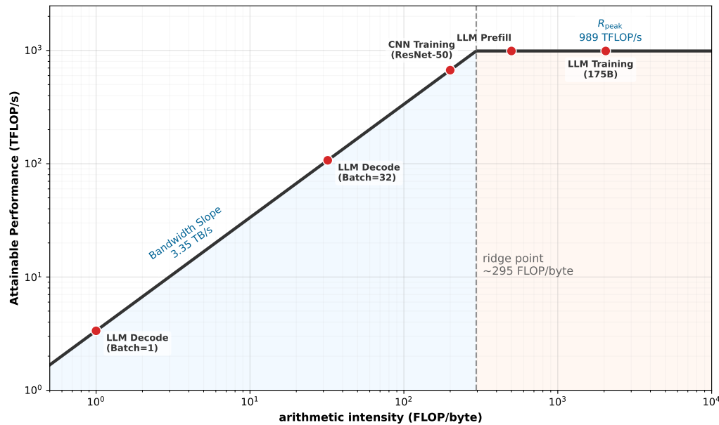
Figure 2.8: The Roofline Landscape: NVIDIA H100 (FP16): H100 roofline showing the memory-bandwidth and peak-compute ceilings, with representative ML workloads spanning memory-bound and compute-bound regions.
