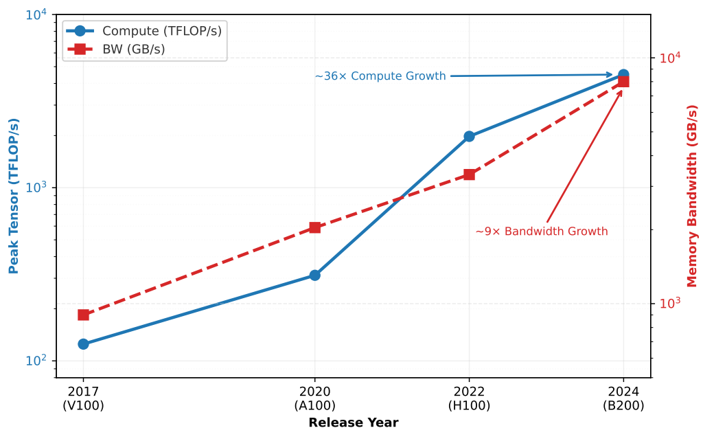
Figure 2.7: The Compute-Memory Divergence: GPU peak Tensor throughput has grown approximately 36\times from V100 to B200 when following each generation's advertised low-precision Tensor Core mode, while HBM bandwidth has grown only 9\times over the same period. The widening gap between these curves is the memory wall: each generation of accelerator becomes proportionally more starved for data.
