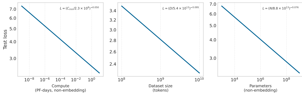
Figure 15.4: Model Scaling Laws: In the ranges studied by Kaplan et al. (2020), increasing model size, dataset size, and compute consistently reduced test loss. The figure reproduces source-paper notation, where N denotes parameter count and C_{min} denotes compute; elsewhere this book uses P for parameter count and O for operation count. These scaling laws explain why larger models, more data, and increased compute became attractive design choices within that regime.
