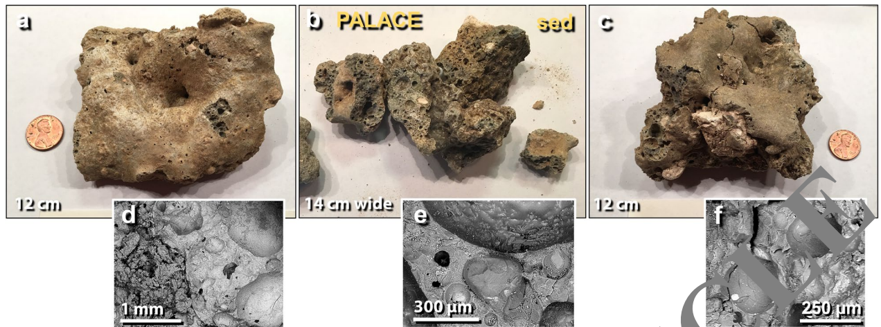
Figure 11. Melted mudbrick from the palace. (a) The upper surface of meltglass showing non-vesicular 'skin'; (b) broken surfaces of meltglass displaying vesicular texture; (c) upper surface and broken faces of meltglass. Note large unmelted light-colored mineral inclusion. (d)–(f) SEM images of highly vesicular surfaces of broken meltglass. Note bright metallic inclusions in several vesicles.
