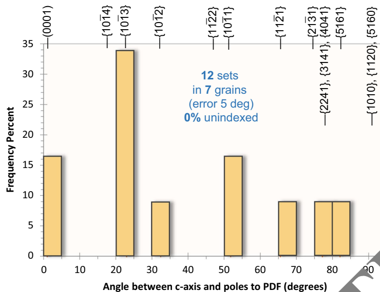
Figure 20. Sets of lamellae in shocked quartz grains. 7 TeH grains/crystals display 12 sets of lamellae in 5° bins; no lamellae were unindexed. Two grains have a set of lamellae {0001} with its pole parallel to the c axis.
